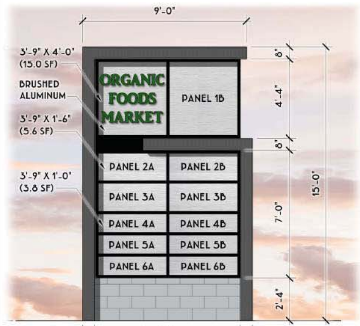
1 MONUMENT SIGN SCALE: 3/16" = 1'-0"
